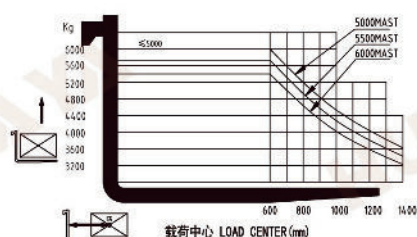
6.0T载荷曲线图 6.0T load curve
