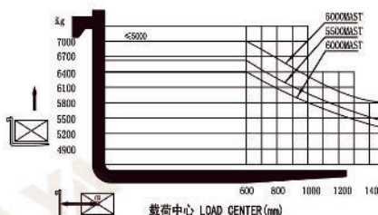
7.0T载荷曲线图 7.0T load curve
