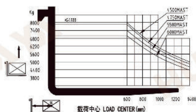
8.0T载荷曲线图 8.0T load curve
