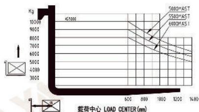
10T载荷曲线图 10T load curve
