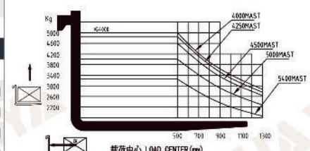
5.0T载荷曲线图 5.0T load curve
