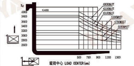
4T载荷曲线图 4T load curve
